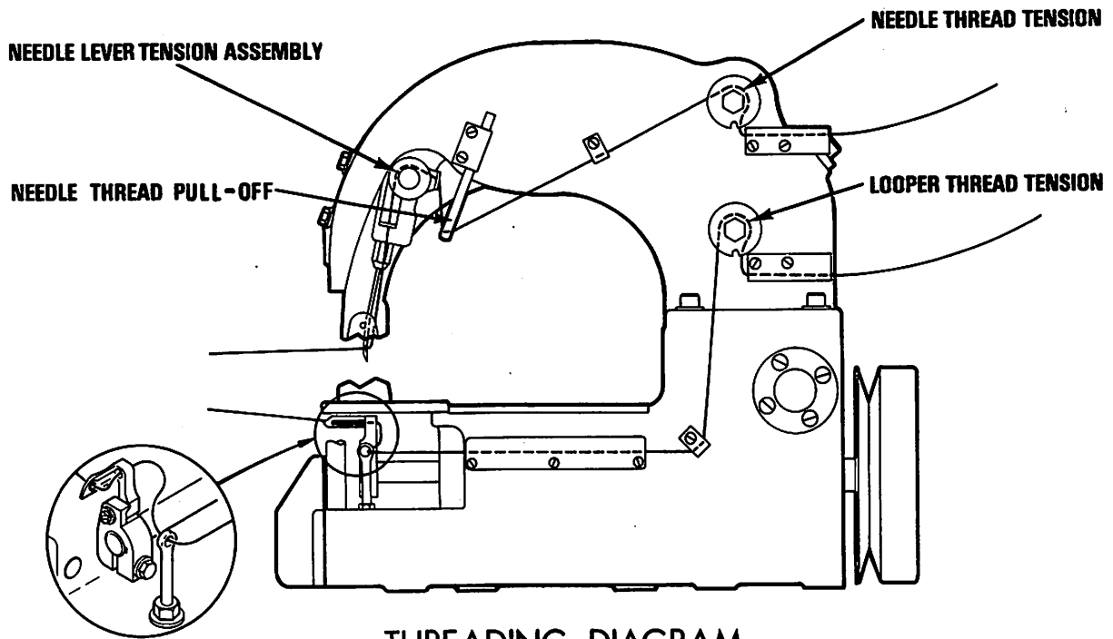
THREADING DIAGRAM
